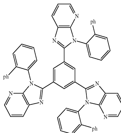
Compound B:
